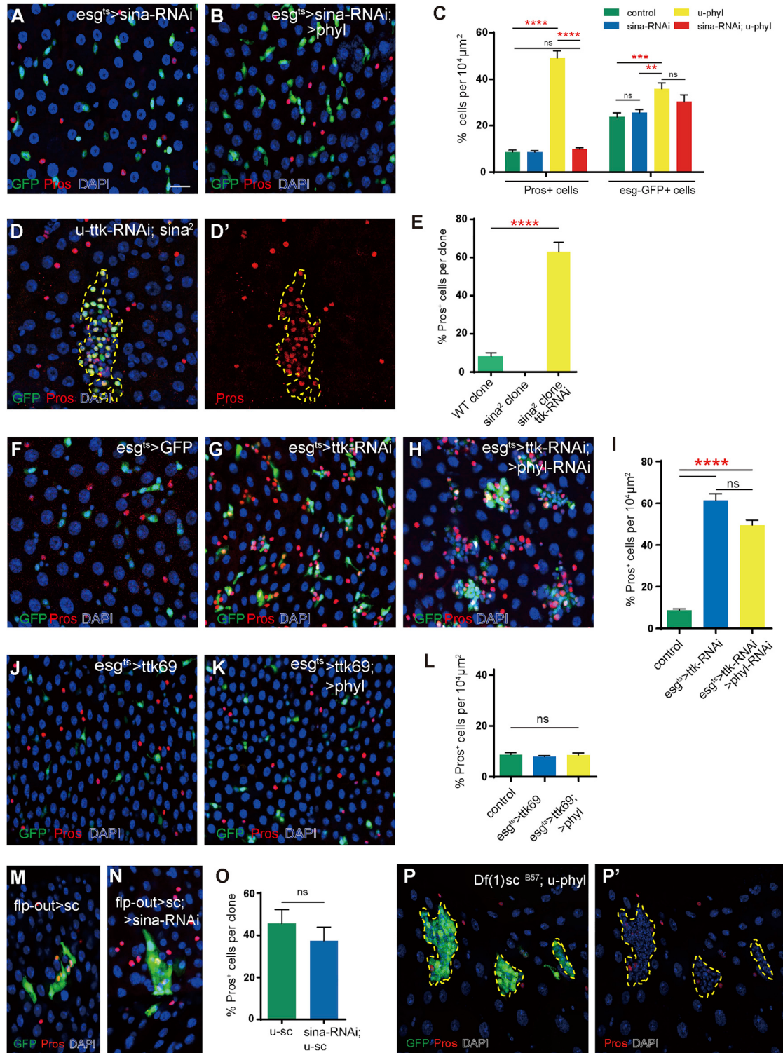
Figure 3. Epistatic Relationships among Sina, Phyl, Ttk69 and AS-C complex in Regulating EE Specification
