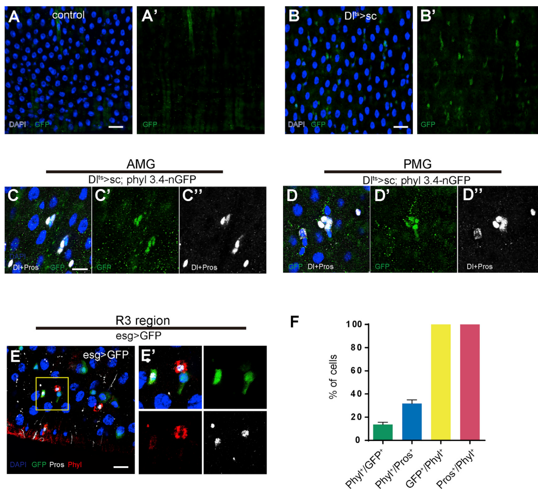
Figure 5. Phyl Is Transiently Upregulated in EE Progenitor Cells and Is Positively Regulated by Sc
