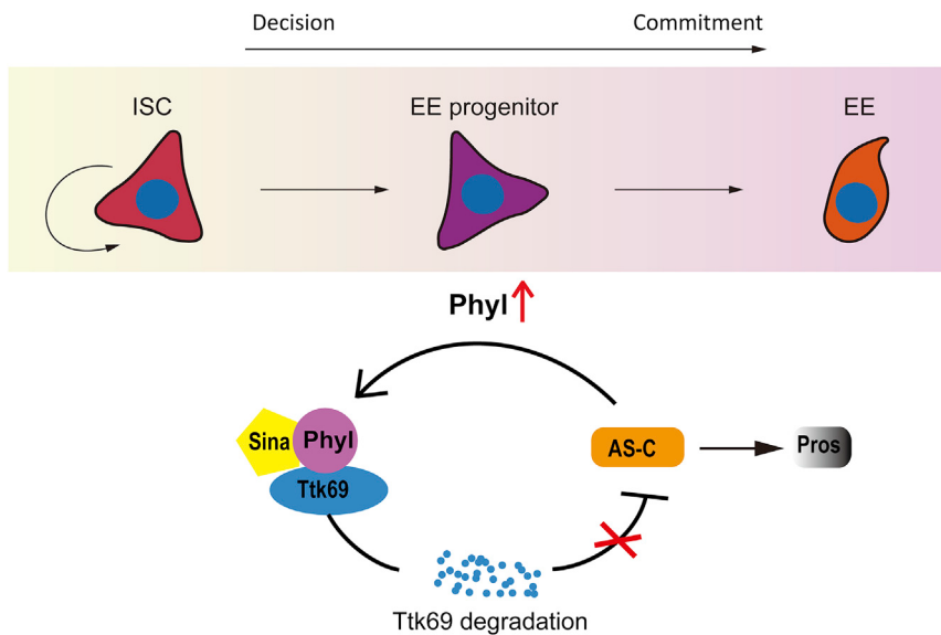
Figure 7. A Schematic Model for EE Specification Driven by the Positive Feedback Regulatory Circuit Composed of Sina/Phyl, Ttk69, and Sc
