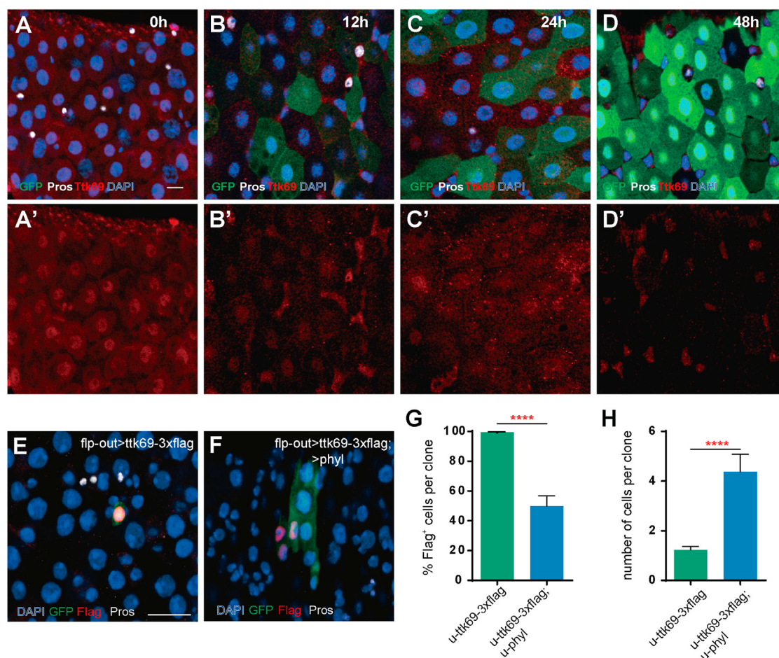
Figure 4. Sina and Phyl Regulate Ttk69 Protein Stability
